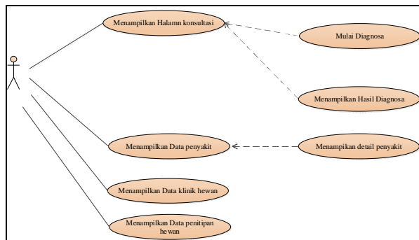
Gambar 3.2 Use Case Diagram User
