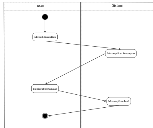
Gambar 3.4 Activity diagram konsultasi
