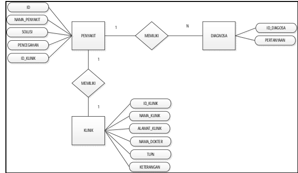
Gambar 3.7 ERD (Entity Relationship Diagram)
