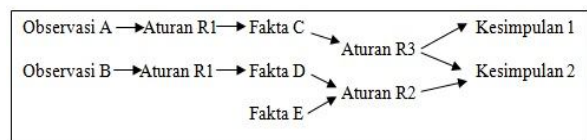
Gambar 2.2 Proses Forward Chaining
