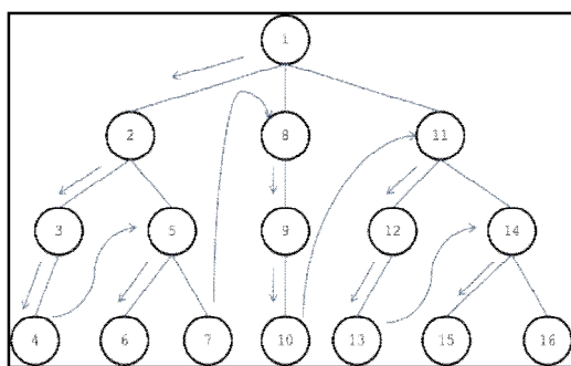
Gambar 2.4 Penelusuran Depth First Search
