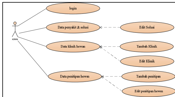
Gambar 3.3 Use Case Diagram Admin
